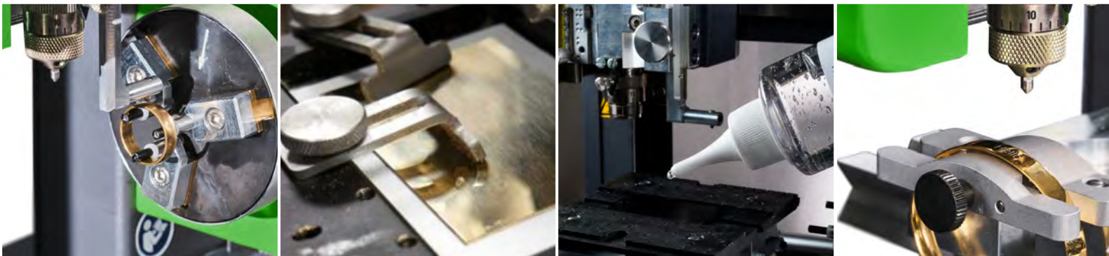
Rotary device Cutting jig Engraving gel Jigs & Holding devices
